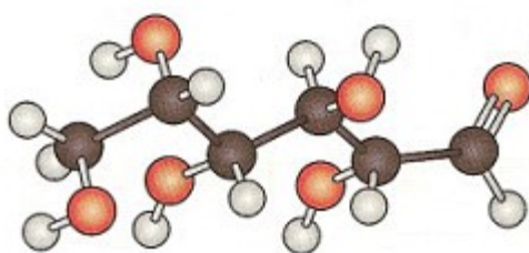
glucose
