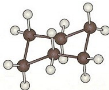
cyclohexane
