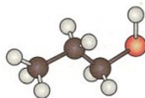
propan-1-ol
